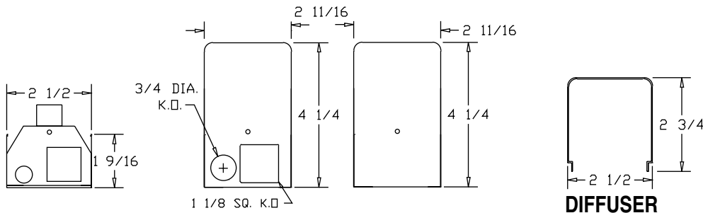
END PLATE
